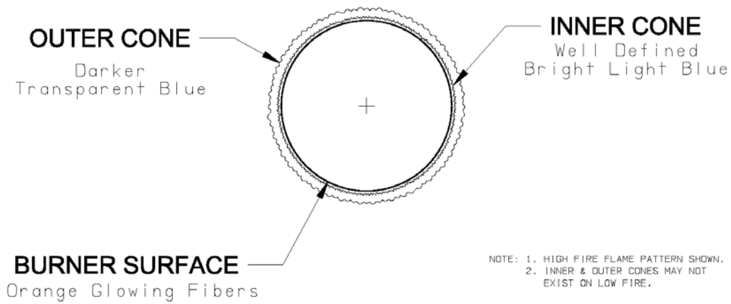
Figure 3: Burner Flame
